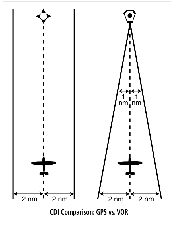
Full-Scale deflection and defined path for normal approach
