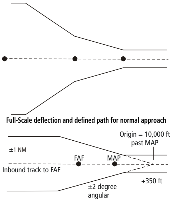
Full-Scale deflection and defined path for VTF approach
